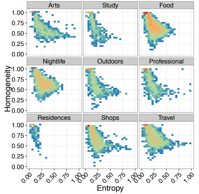
Figure 5: Entropy vs homogeneity distribution per category. Colour gradient reflects the frequency of observation with red being high and blue being low.
