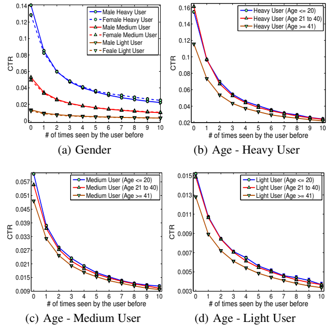
Figure 6: User Demographics
