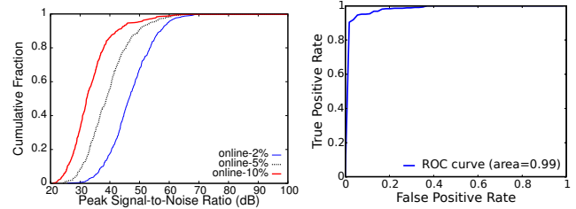
Figure 9: PSNR (dB) between the rendered video and the non-backlight-scaled video. Figure 10: The ROC curve for L2 storyboard predictions of power savings under online-10%.
