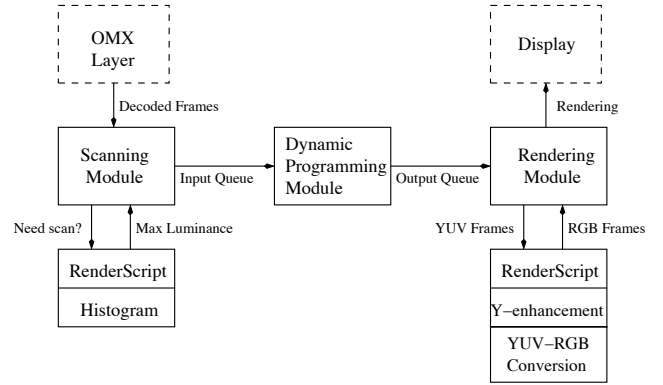
Figure 4: The organization of our GoCAD-enabled Android application.
