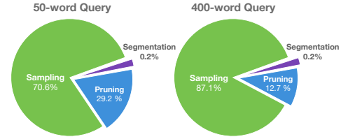
Figure 7: Breakdown of query processing time
