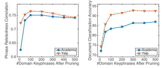
Figure 5: Performance variations of LAKI with increasing number of keyphrases
