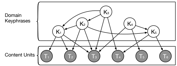
Figure 2: An illustrative Bayesian network for domain keyphrase silhouetting.
