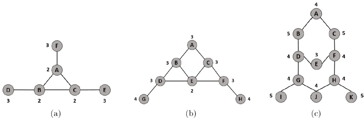
Figure 2: Three graphs with different eccentricity functions. The number next to each vertex indicates its eccentricity. (a) A graph with a unimodal eccentricity function. (b) A graph with a non-unimodal eccentricity function. (c) A graph with a non-unimodal eccentricity function.
