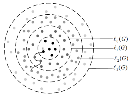
Figure 1: Eccentricity Layering of a graph.
